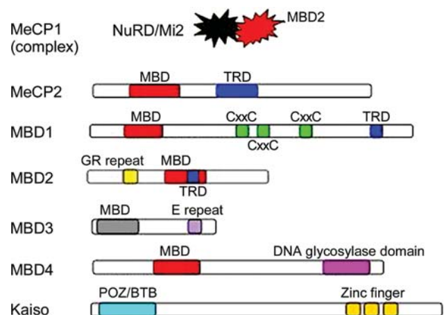
Figure 3 Maps of methyl-binding proteins NuRD/Mi2 is a complex. MBD, methyl-binding domain; TRD, transcriptional repression domain; CxxC, cysteine-rich domain; GR repeat, glycine and arginine repeat; E repeat, glutamate repeat. All of them except MBD3 have the ability to bind methylated DNA. POZ/BTB, Pox virus and zinc finger/bric-a-brac tramtrack broad complex (POZ/BTB) motif. Gray indicates the inability of MBD3 to bind methylated DNA. Kaiso recognizes methylated DNA via zinc finger instead of MBD.
