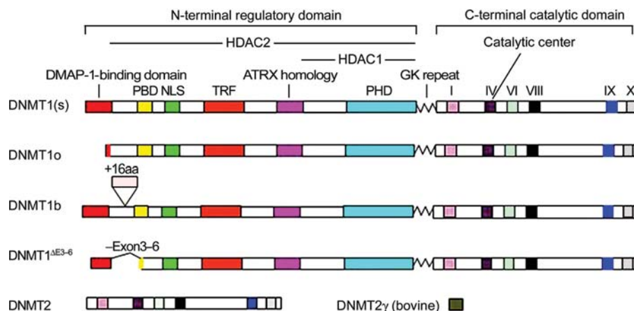
Figure 1 Schematic drawing of the architecture of human DNMT1, DNMT2 and their splicing isoforms with the exception of bovine DNMT2 \gamma . PBD, PCNA-binding domain; NLS, nuclear localization signal; TRF, targeting replication foci; ATRX homology, also known as Cys-rich-region, namely zinc-binding motif; PHD, polybromo-1 homology domain; GK repeat, glycine-lysine repeat; the remaining are the six most conserved motifs, with catalytic center located in motif IV. Interaction domains of HDAC1 and HDAC2 are indicated. DNMT2 only consists of C-terminal catalytic domain. DNMT2 \gamma just has 63 amino acids via a premature stop codon.
