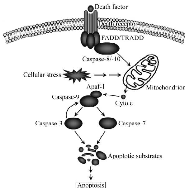
Fig. 3 Typical mitochondrion-mediated and caspase-dependent pathway Apaf-1, apoptotic protease activation factor-1; Cyto c, cytochrome c; FADD, Fas-associated death domain; TRADD, tumour necrosis factor receptor-associated death domain.
